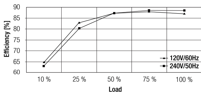
LCU 150/0012 E020 – Efficiency versus load
