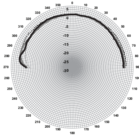
LC1-UM24E8 Frequency response
