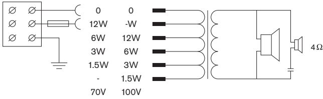
LC1-UM12E8 Circuit diagram
