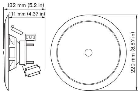
LC1-WM06E8 Dimensions in mm (in)
