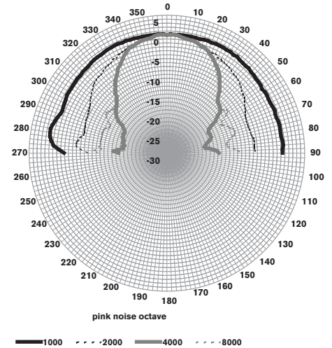
LC1-UM12E8 Polar diagrams
