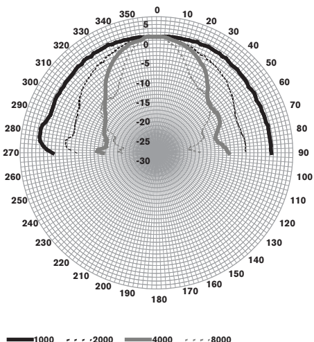
LC1-UM06E8 Polar diagrams
