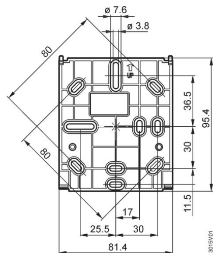
Base plate
