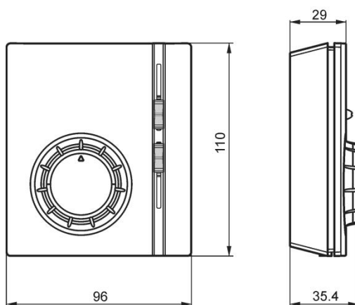
Room thermostat
