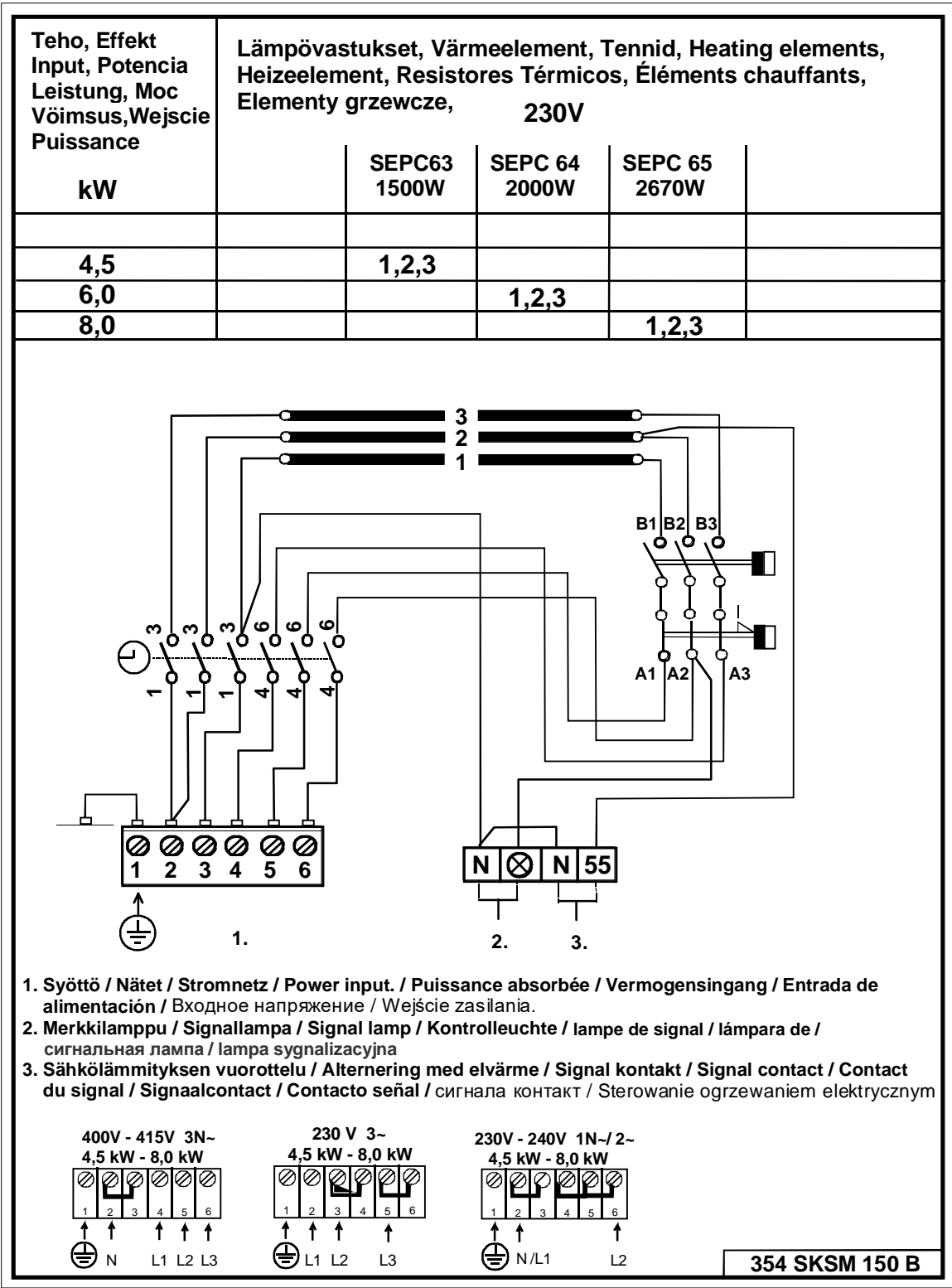
Image 4 Viring diagram
