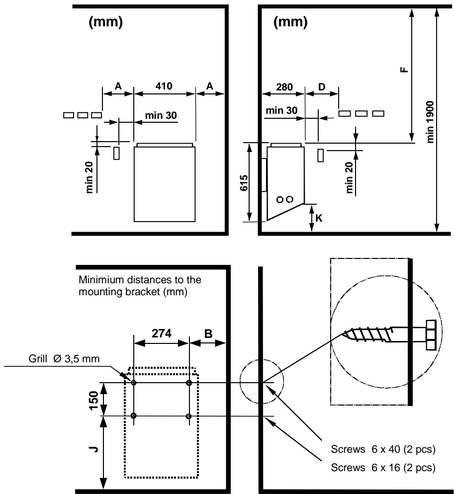
Image 2 Safety clearances
