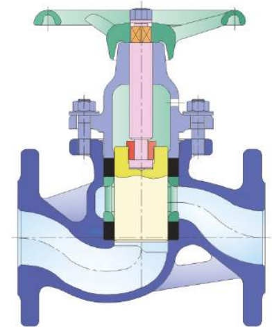
YPG 15-50
